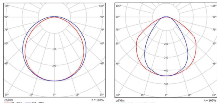
Wide Beam
