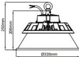
Universal Reflector
