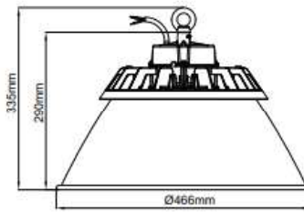
Tall Reflector
